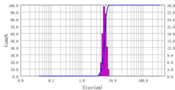
图2 激光衍射粒度分布/ Laser Diffraction PSD
